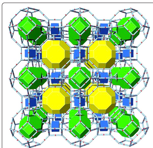
Figure 2 Zeolite A structure: an assembly of framework's cages (tiles). Centre of a tile is the centre of a void in the framework. Voids are connected with adjacent ones through the large "windows" which are faces of tiles.
