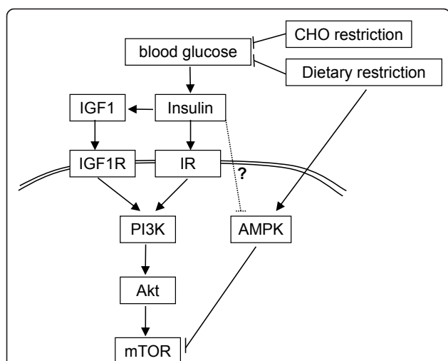
Figure 2 The IGF1R-IR/PI3K/Akt/mTOR pathway and its manipulation through diet.
